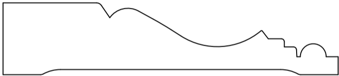
HWP1232 Casing 0.750" x 3.500"
