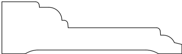
HWP1203 Casing 0.875" x 3.000"
