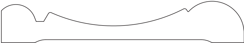
HWP1193 Casing 0.750" x 4.375"
