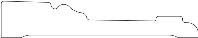
HWP1181 Casing 0.750" x 4.000"
