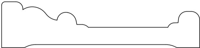
HWP1148 Casing 0.812" x 3.500"
