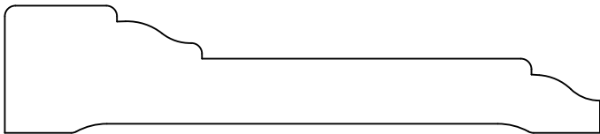
HWP1061 Casing 0.750" x 3.500"
